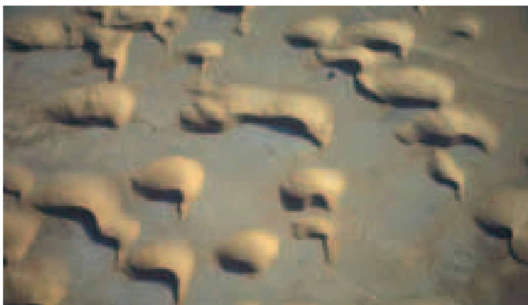
Isolated barchans
