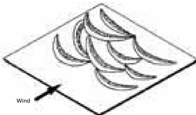
FIGURE 8 Aklé dune
