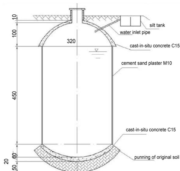
Profile of a 40 cubic meters cement-shell water cellar
