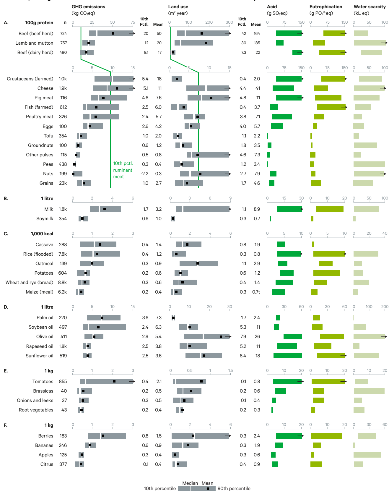
Figure 7. Estimated global variation in GHG emissions, land use, terrestrial acidification, eutrophication and scarcity-weighted freshwater withdrawals, within and between 36 major foods
