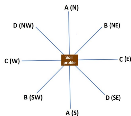
Figure 10: Sampling design
