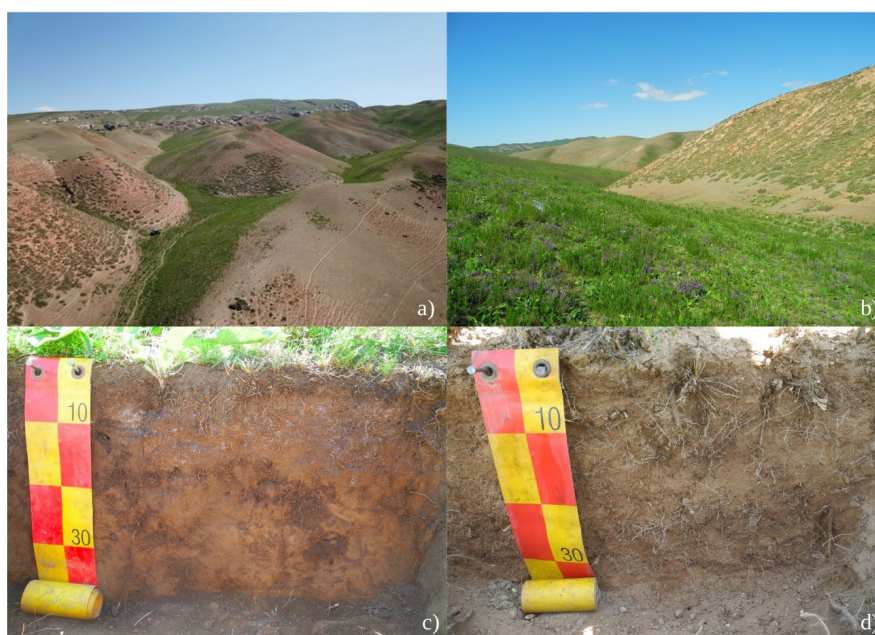
Figure 1: Kyrgyz grassland location with a densely vegetated northern slope and sparse vegetation on the southern slope, a) from above, b) in the area, c) soil profile on the northern slope, d) soil profile on the southern slope
