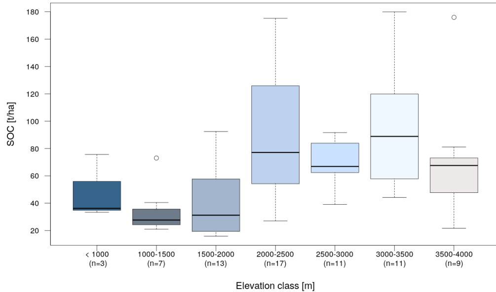
Figure 13: Relationship between elevation class and soil organic carbon stocks in tonnes per hectare
