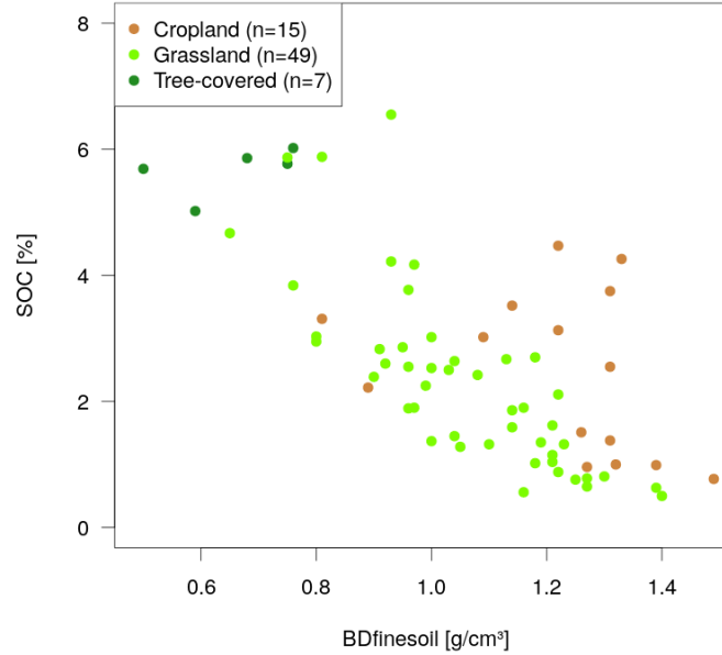
Figure 15: Relationship of soil organic carbon content [%] and bulk density of the fine soil [g/cm³]
