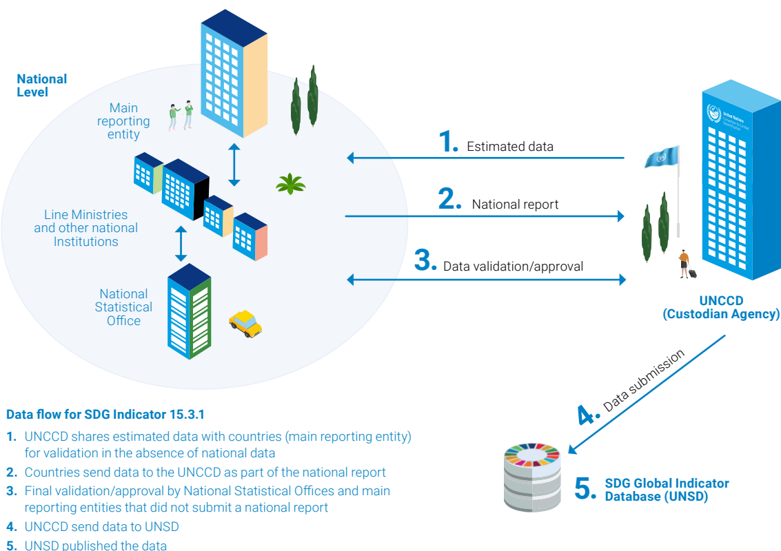
Figure 2-3 Data flow for SDG Indicator 15.3.1
