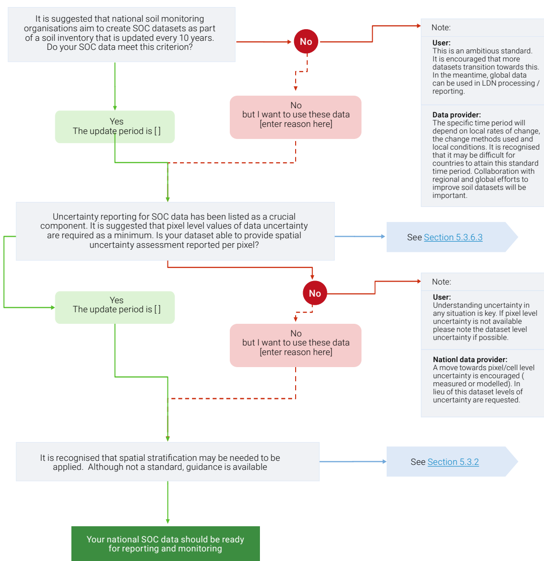
Figure 5-1 Decision tree for determining the most appropriate data for calculation of the soil organic carbon stock change sub-indicator (from GEO-LDN Initiative, 2020).
