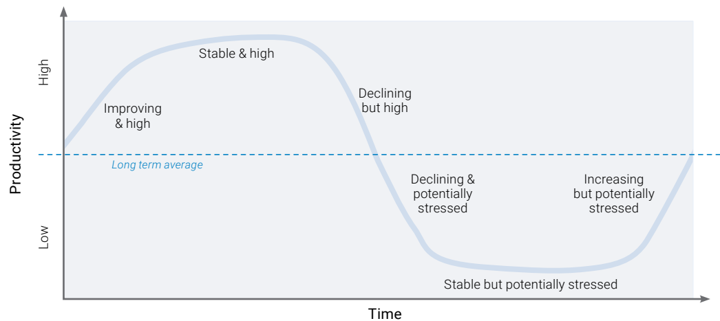
Figure 4-2 Stylised phases in the long-term average trend of land productivity. A declining trend of productivity, or productivity levels that remain below the long-term average, may indicate productivity degradation.
