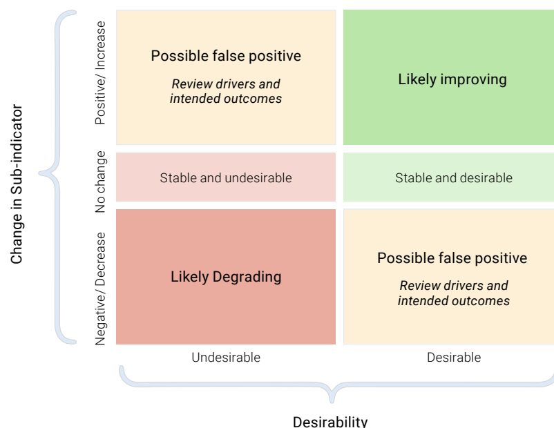
Figure 2-4 Generic degradation interpretation matrix for any sub-indicator of Indicator 15.3.1. The ‘Increase’ and ‘Decrease’ y-axis labels should be used for the Land Productivity and SOC sub-indicators, and the ‘Positive’ and ‘Negative’ labels for Land Cover. (Sims et al., 2020)
