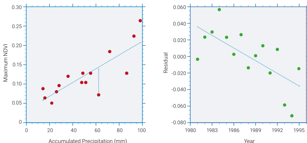
Figure B-1 Linear regressions between (a) accumulated precipitation and the maximum NDVI – the residual is illustrated by the line, and (b) the temporal trend of associated residuals (source Evans and Geerken 2004).
