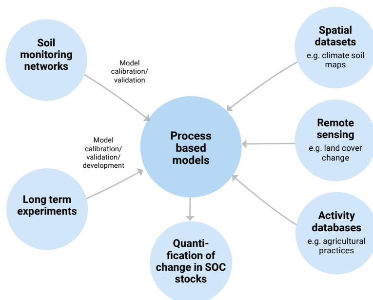
Figure 5-2 Schematic of possible national Tier 3 approach for estimating change in soil organic carbon stock.
