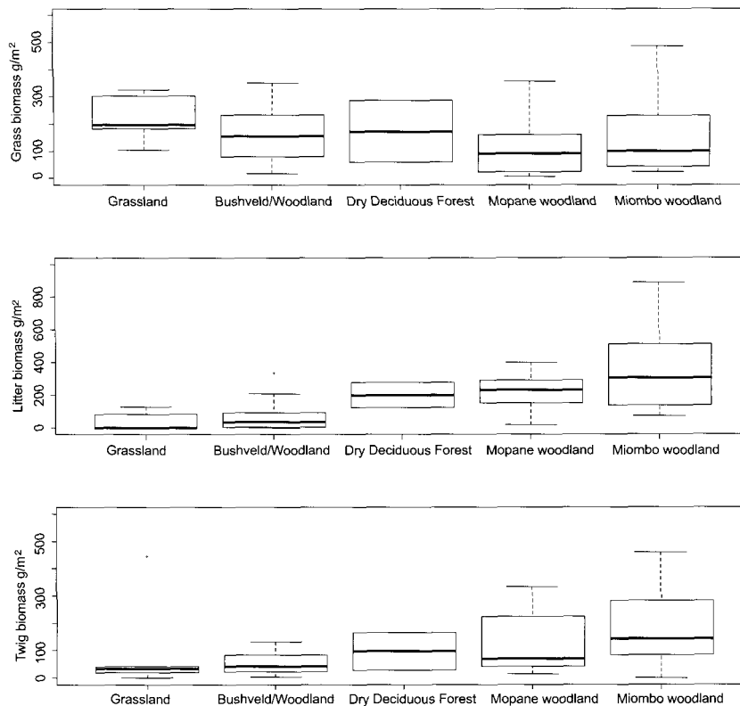
Fig. 3 Biomass of grass, litter and twig fuels for different vegetation types in southern Africa in order of generally increasing tree fraction cover. Data represent summaries from ~60 field measurements across southern Africa. Mean annual rainfall for the sites in each vegetation type: grassland – 740 mm, bushveld/woodland – 720mm, dry deciduous forest – 641 mm, mopane woodland 616mm, miombo woodland, 885 mm. Bushveld/woodland is a low (~5m tall), deciduous woodland, often dominated by trees from the family Combretaceae. Mopane woodland is a 2-10 m tall deciduous woodland highly dominated by Colophospermum mopane . Miombo woodland is a tall (~10 m) deciduous woodland containing many species, but typically dominated by trees from the genus Brachystegia .
