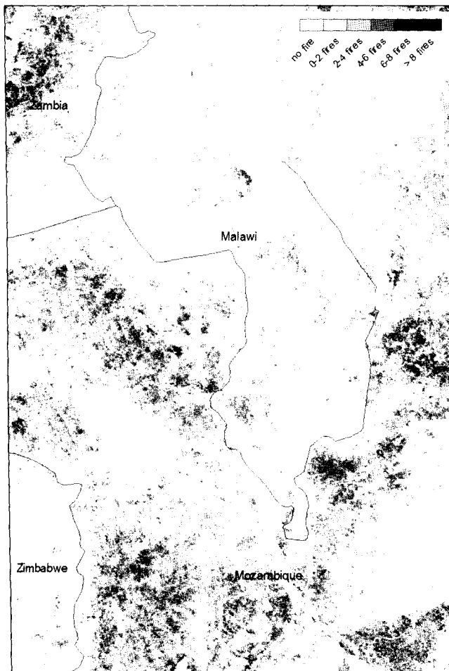
Fig. 2 Number of fires over an eight-year period in a heavily-utilised rural landscape in Malawi. The patches of the landscape that burn do so repeatedly, but most of the landscape remains unburned. This means that using fire return times to estimate burned area becomes problematic: the Mean Return Interval (MRI) for fires in Malawi is 3-4 years (Archibald, 2010) which would produce a burned area estimate of 20-30%. In reality, less than 10% burns every year.
