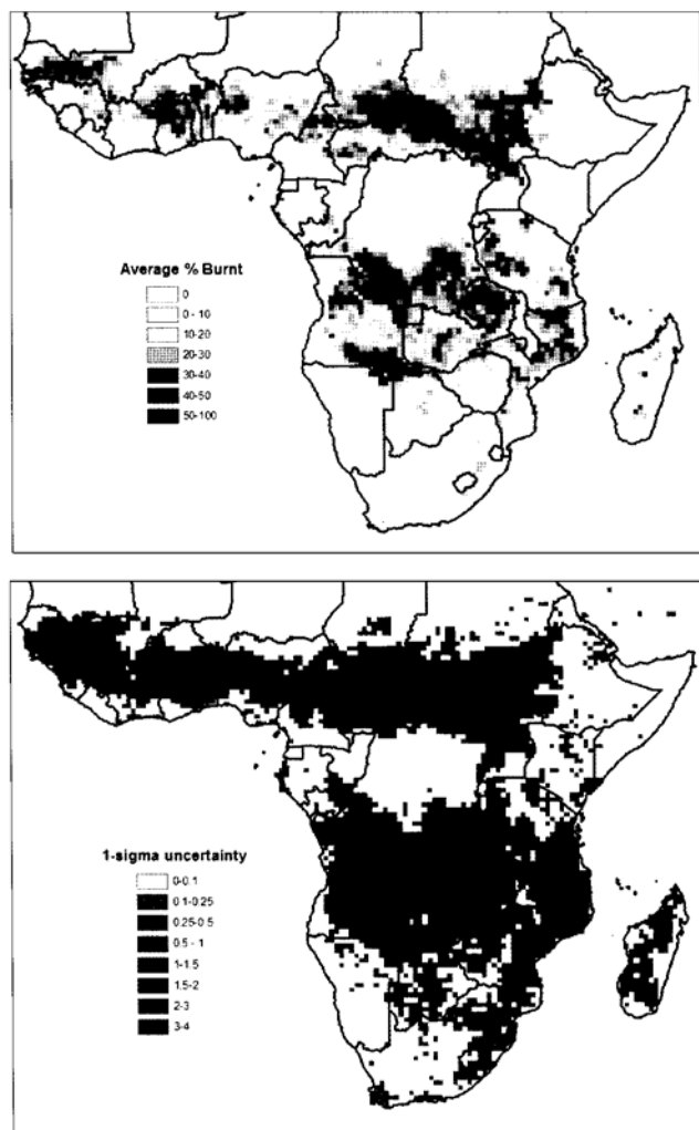
Fig. 1 Map of average burned area fraction in sub-Saharan Africa over twelve years, and associated uncertainty ( 1-\sigma ) derived from the GFED3 dataset (Giglio et al. , 2010) at 0.5 degree resolution. The unburned area around the equator is rainforest, too wet to burn on a widespread basis.
