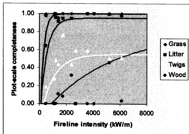
Fig. 4 Combustion completeness in different categories of fuel observed in savanna fires in southern Africa (data from Shea et al. , 1996). The fireline intensity is the rate of energy release along the burning edge of a fire.
