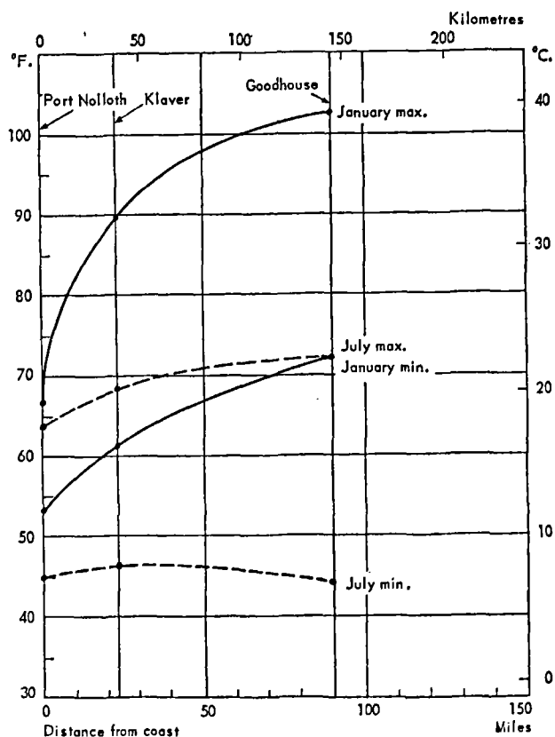
FIG. 6. Profiles of mean daily maximum and minimum temperatures, south-western Africa.
