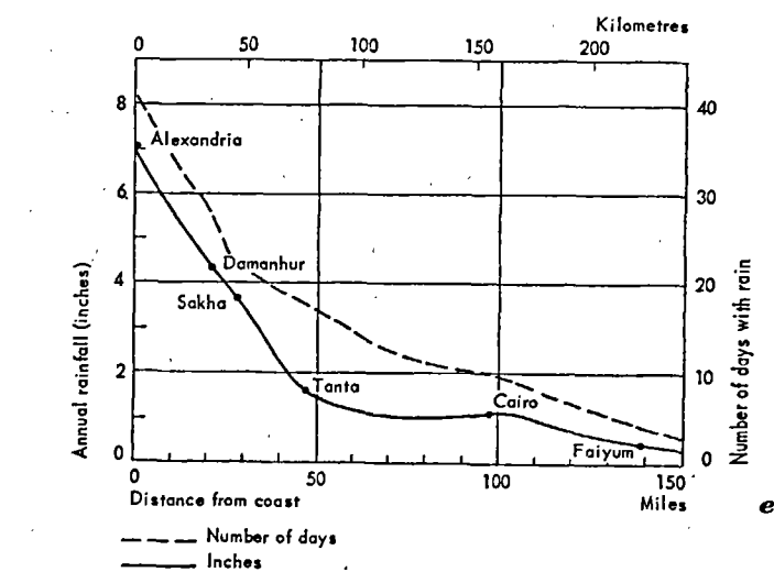
FIG. 5. Climatic profiles, Nile Delta.
