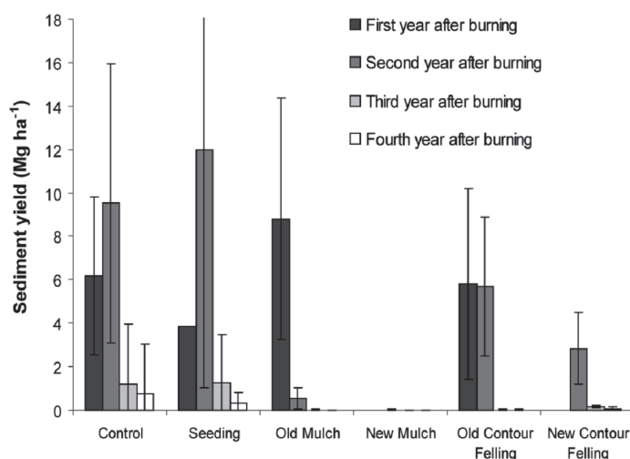
FIGURE 9. Annual sediment yields from treated and control hillslopes at the Bobcat fire. Old much and old contour felling refer to treatments that were applied before a very large storm that occurred two months after the fire. New mulch and new contour felling refer to treatments applied after this storm. Bars indicate one standard deviation.
