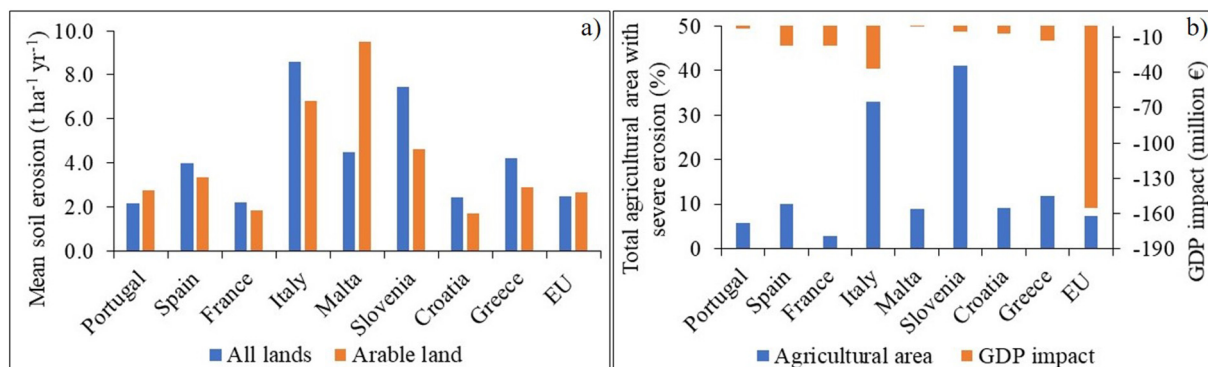
Fig. 6. a) Mean soil erosion in the EU Mediterranean countries (adapted from Panagos et al., 2020); and b) percentage of total agricultural land suffering severe soil erosion ( > 2 \text{ t ha}^{-1} \text{ yr}^{-1} ) and impact on GDP due to productivity loss (adapted from Panagos et al., 2018b).
