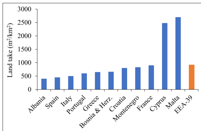
Fig. 4. Land take in the European Mediterranean countries, 2012-2018. (Adapted from EEA, 2019b.)
