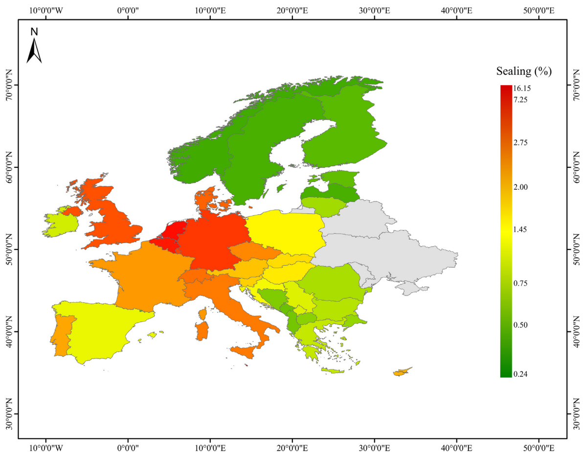
Fig. 5. Percentage soil sealing in different European countries in 2015.
