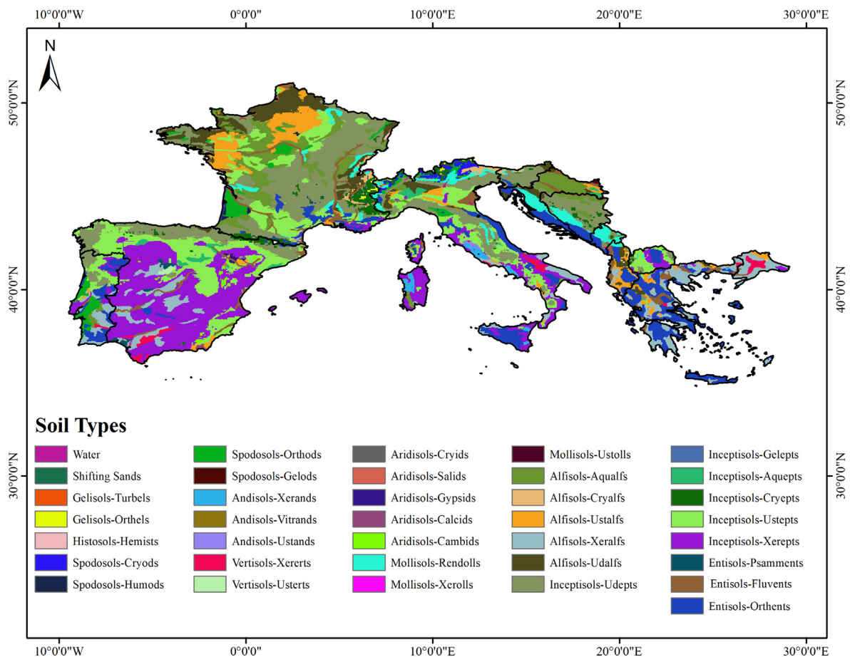
Fig. 3. Major soil types in the EU Mediterranean countries.
