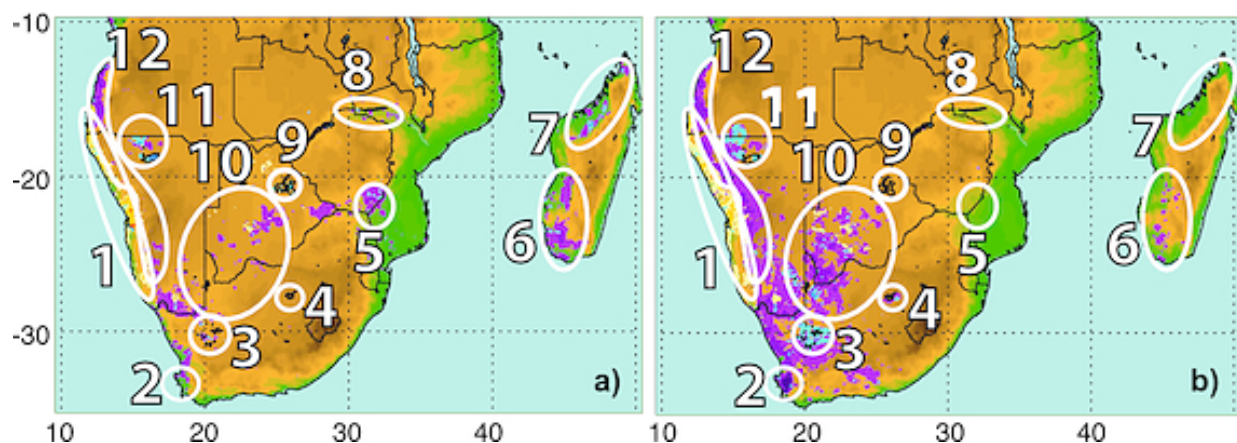
Figure 3.8: Distribution of the percentage number of days per season (a: September, October, and November; and b: December, January, and February) with Dust Optical Depth > 0.2 over Southern Africa. The colour shadings are the same as in Figure 3.5. The white circled source areas are numbered as follows: 1, Namib Desert; 2, croplands near Cape Town in South Africa; 3, South African Bushmanland; 4, Bloemhof Dam of South Africa; 5, Hippo Valley of Zimbabwe; 6, southern Madagascar; 7, northern Madagascar; 8, Cahora Bassa reservoir of Mozambique; 9, Makgadikgadi Pans of Botswana; 10, Kalahari Desert; 11, Etosha Pan; and 12, Great Escarpment of Namibia. Source: Ginoux et al. (2012).
