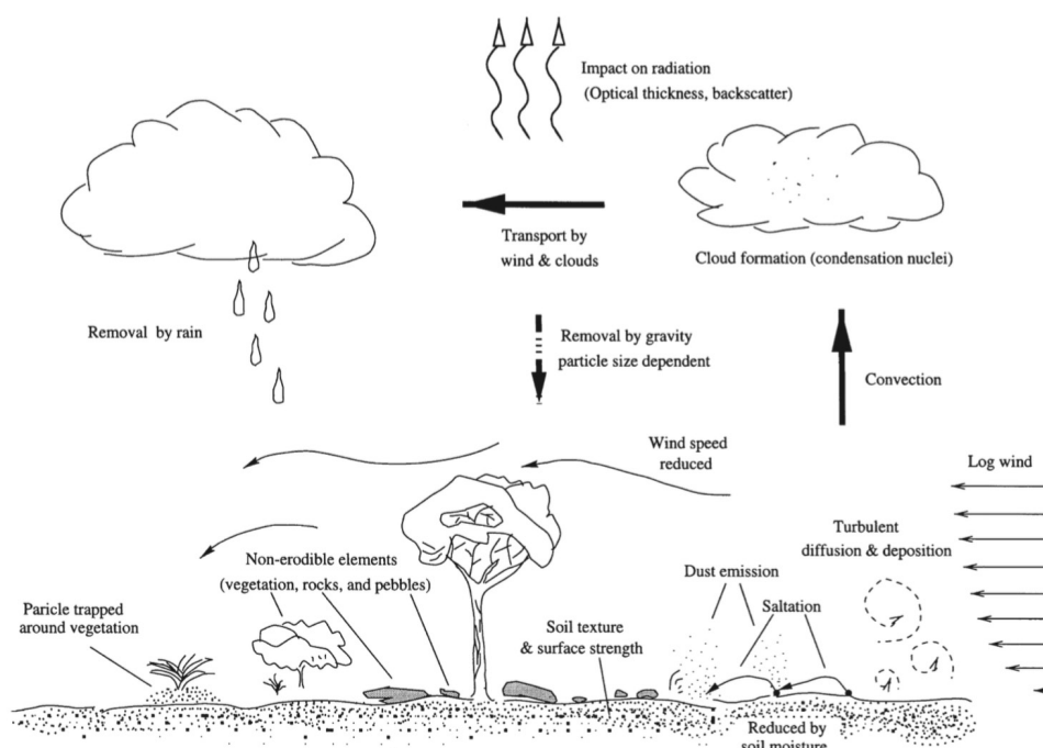
Figure 2.2: A simplified depiction of sand and dust storm processes, controlling factors and impacts. Source: Lu and Shao (2001).
