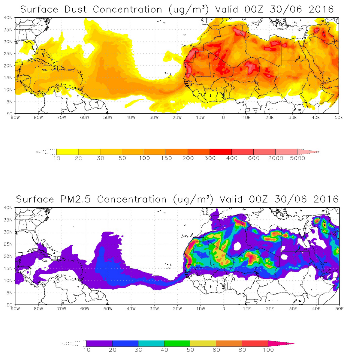
Figure 5.16: Seven-day forecast of (a) near surface dust concentration and (b) surface PM2.5 concentration forecast valid for 00Z, June 30 2016. Source: CIMH (2016).
