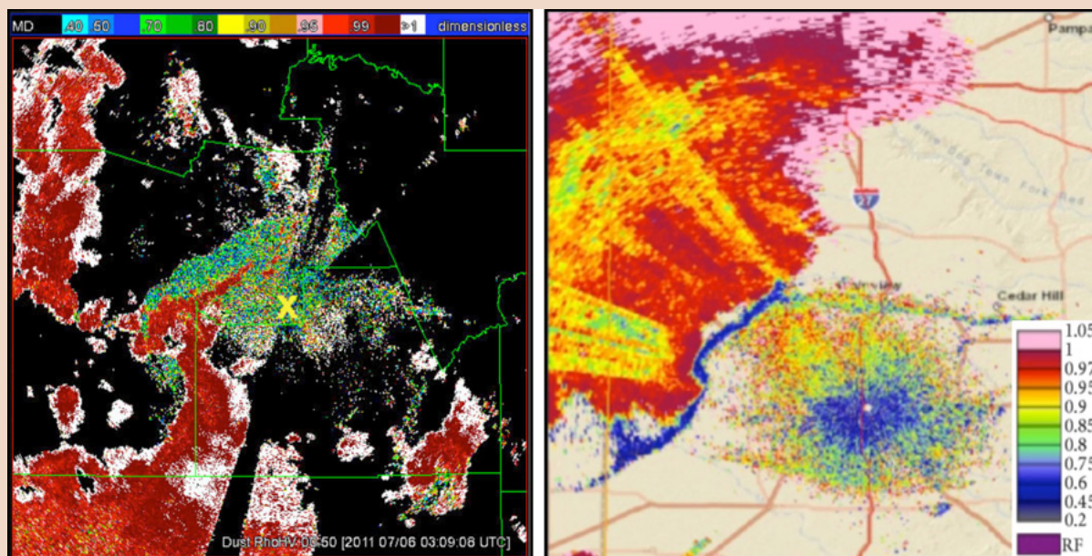
Dual-polarized radar values of correlation coefficient for haboob events: 5 July 2011 Phoenix, AZ (left) and 5 June 2013 Lubbock (TX). Source: Vukovic et al. (2014), Dempsey (2014).
