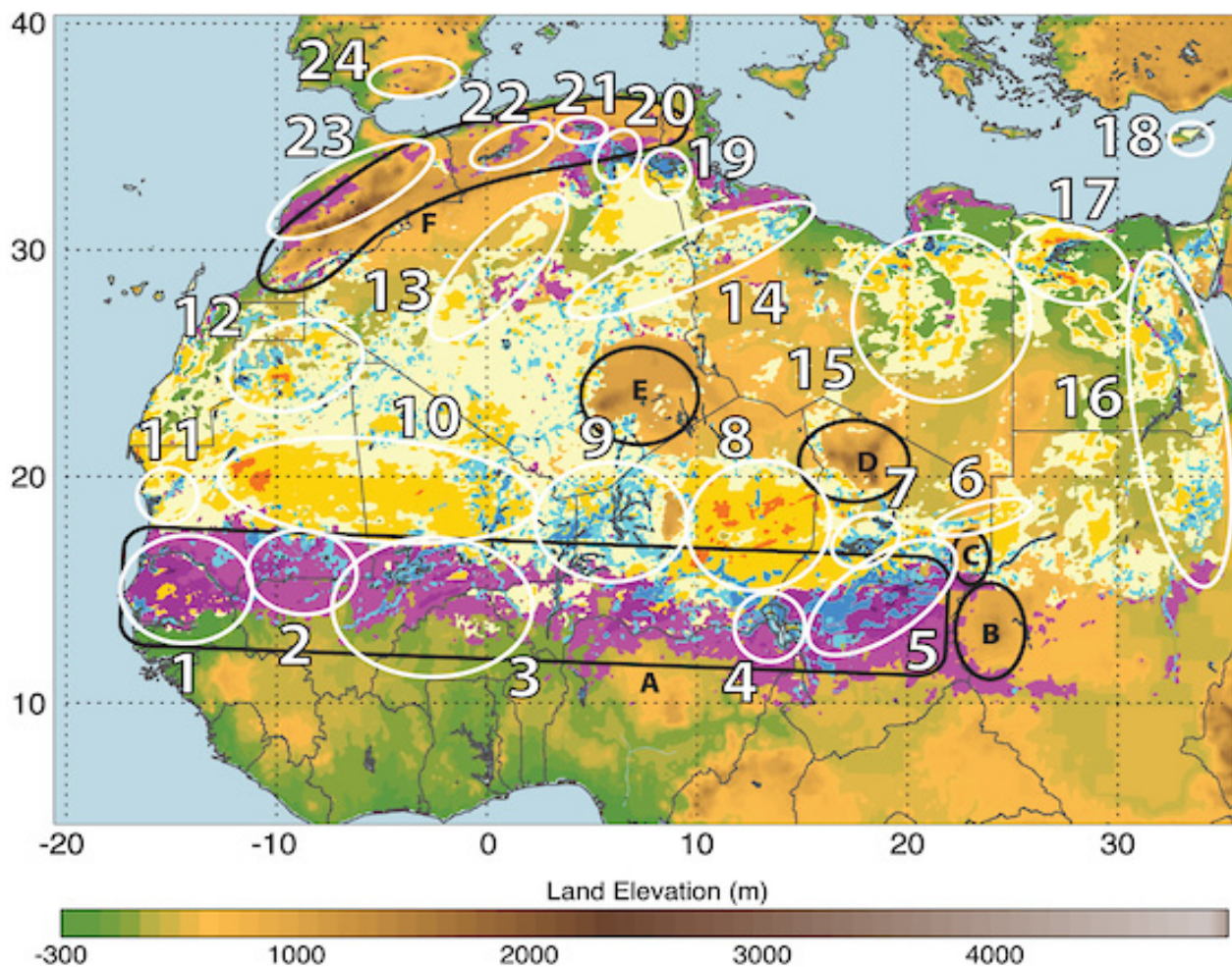
Figure 3.5: Distribution of the percentage number of days per year with Dust Optical Depth > 0.2 over West and North Africa and Southern Europe. The frequencies associated with hydrologic sources are shaded in blue, with natural land use in yellow to red, and anthropogenic land use (more than 30%) in magenta. The frequency levels are 10%, 20%, 40%, 60%, and 100%. Topography shading varies from dark green (300 m) to brown (1000–4000 m), then to grey for high elevation up to 8000 m. The white circled source areas are numbered as follows: 1, Senegal River Basin; 2, Aoukar depression; 3, upper Niger River Basin; 4, Lake Chad; 5, river drainage basin of the Ennedi and Ouaddai highlands; 6, Mourdi depression; 7, Bodélé depression; 8, Grand Erg of Bilma; 9, river drainage basin of the Aïr; 10, Erg El Djouf; 11, Sebkhet te-n-Dgâma; 12, Tiris Zemmour region; 13, Grand Erg Occidental; 14, Grand Erg Oriental; 15, Libyan Desert; 16, Nile River Basin; 17, Qattarah depression; 18, Mesaoria plain in Cyprus; 19, Chott el Jerid; 20, Chott Melhir; 21, Chott el Hodma; 22, Chott ech Chergui; 23, Morocco coastal plains; and 24, Andalusia in Spain. Some geographic features are contoured in black and are labeled as follows: A, the Sahel; B, the Ouaddai Highlands; C, Ennedi; D, Tibesti; E, Ahaggar; and F, Atlas Mountains. Source: Ginoux et al. (2012).
