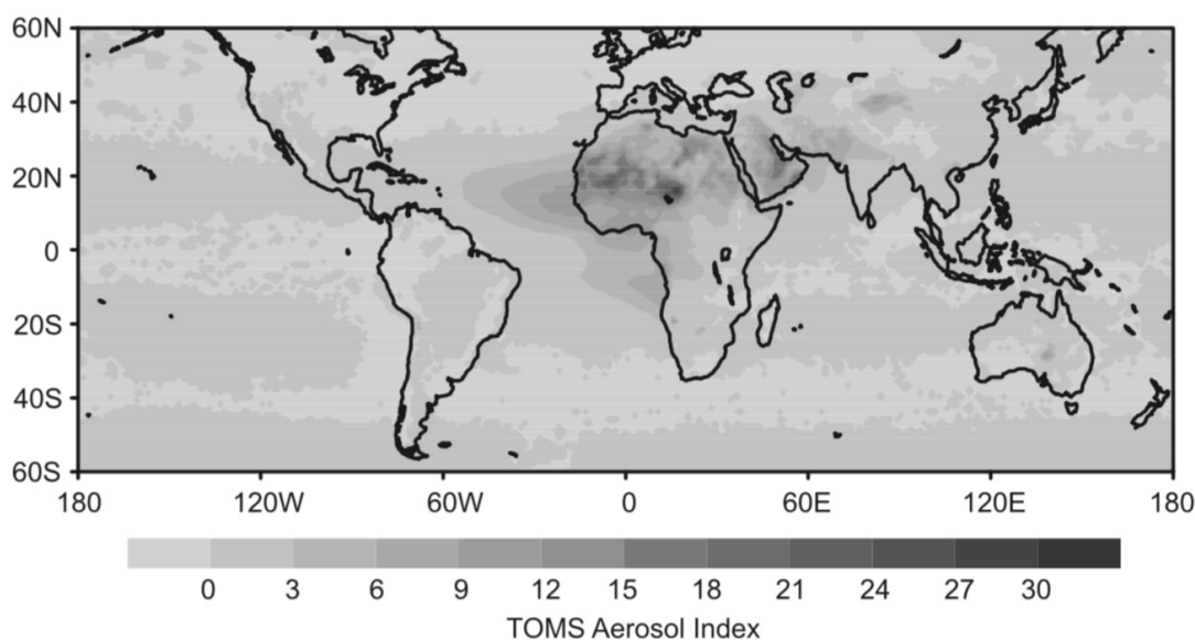
Figure 3.2: The world map of annual mean aerosol index (AI) values (x10) determined by the Total Ozone Mapping Spectrometer (TOMS). Source: Washington et al. (2003)
