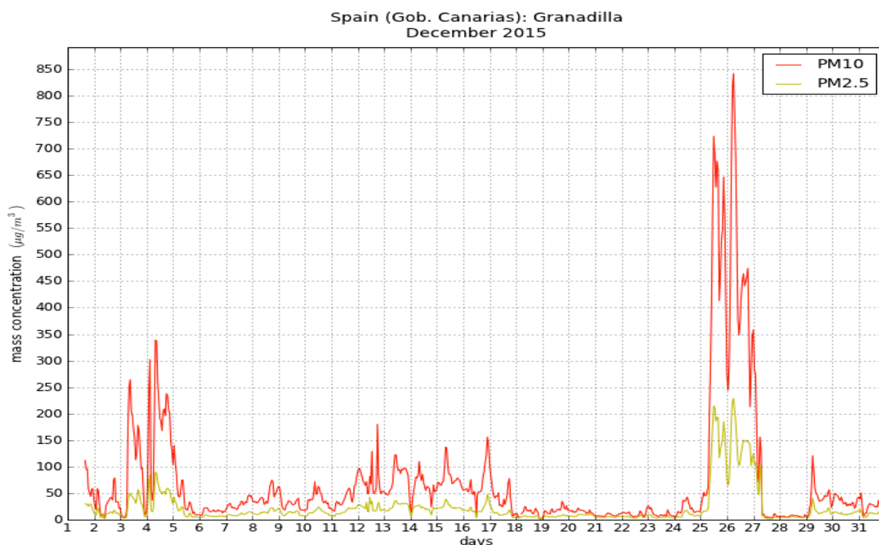
Figure 5.2: The record of particulate matter of 10 \mu\text{m} or less in diameter (PM10) and 2.5 \mu\text{m} in diameter (PM2.5) from Granadilla (Canary Islands, Spain), which clearly shows a major dust event on 25-26 December 2015 and a less significant one on 4-5 December. Source: SDS-WAS.
