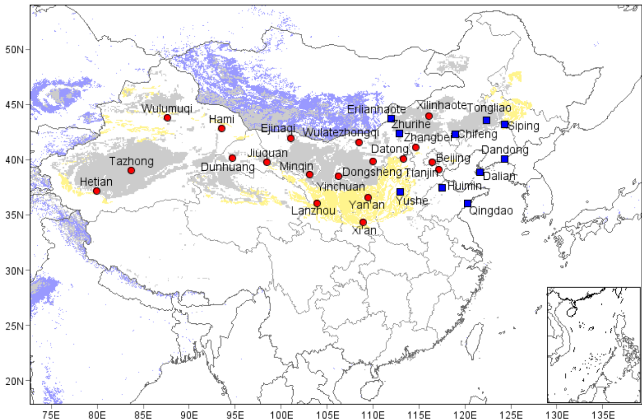
Figure 5.6: Sand and dust storm observation stations of China Meteorological Association, ten of them established from China-Korea cooperation (Blue colour).
