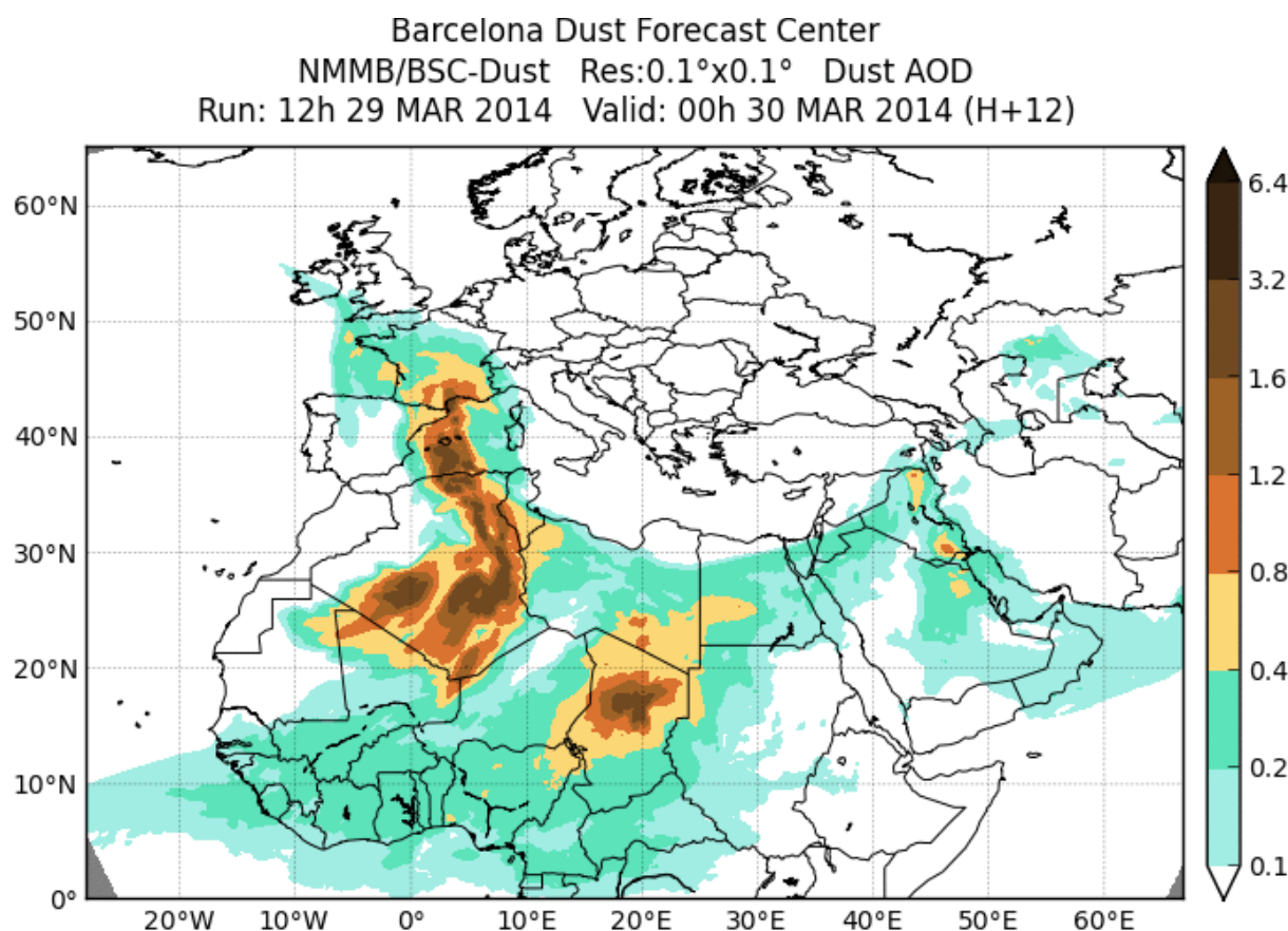
Figure 5.15: H+12 forecast of dust optical depth at 550 nm released by the Barcelona Dust forecast Center on 29 March 2014 at 12 UTC. Source: Barcelona Dust Forecast Center.
