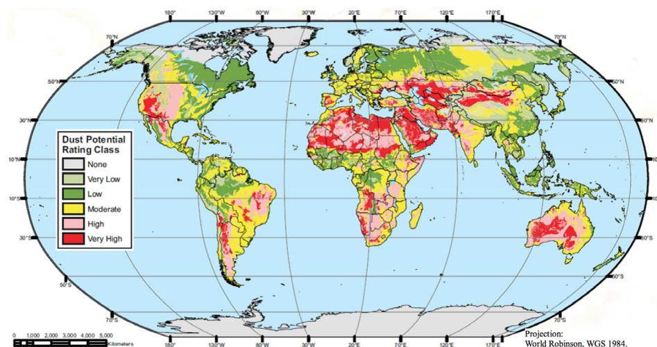
Figure 1.1: Global Dust Potential Map. Source: DTF (2013).
