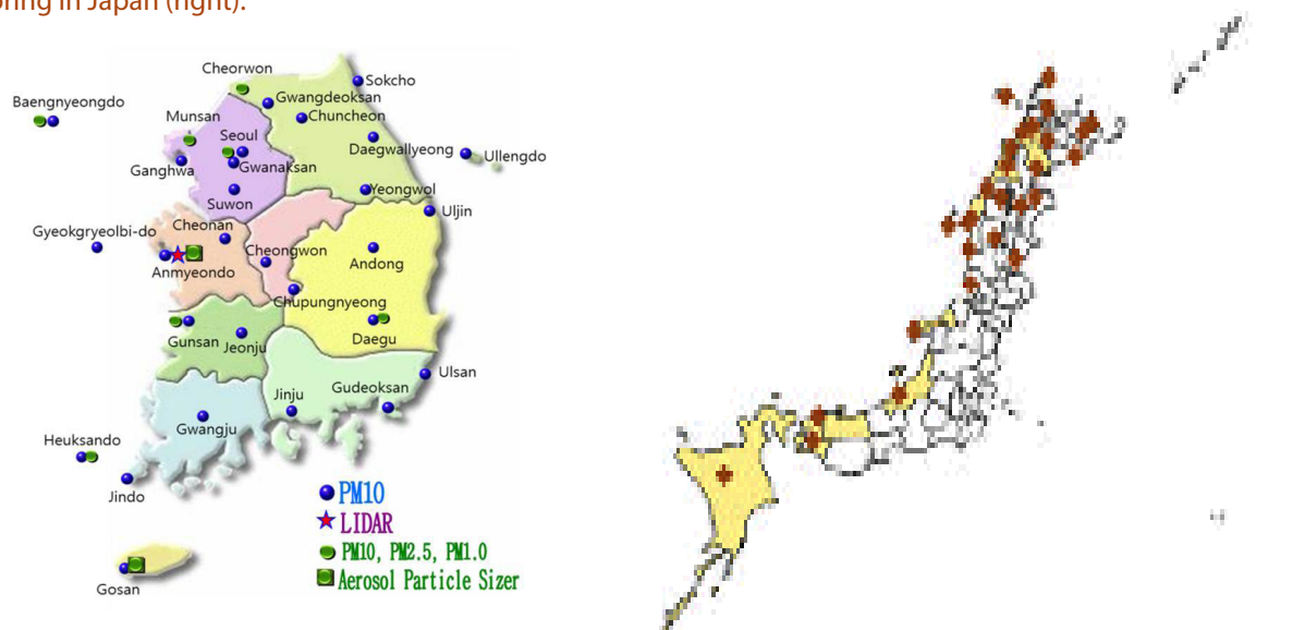
Figure 5.7: Sand and dust storm observation stations of the Korean Meteorological Association (left) and PM 10 monitoring in Japan (right).
