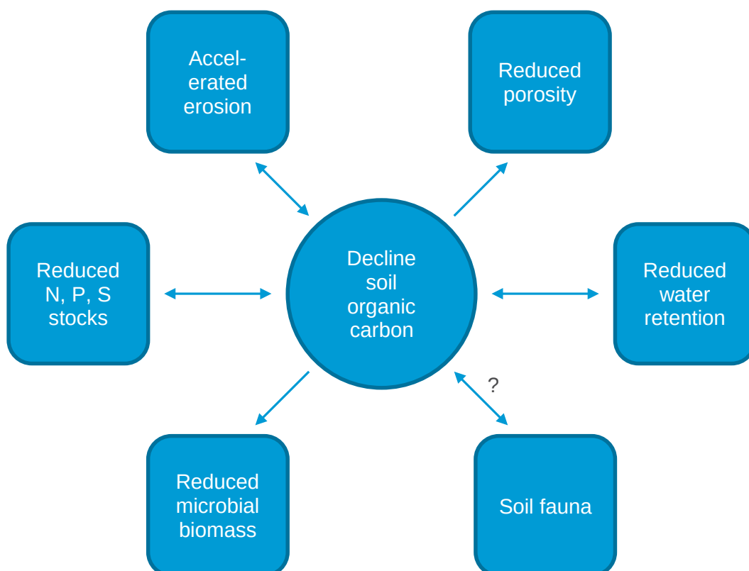
Figure 2: Decline in soil organic carbon stock and soil degradation processes
