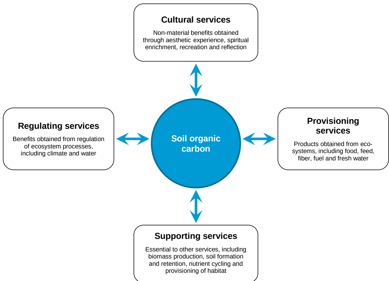
Figure 1: Categories of Ecosystem Services (ESs) underpinned by soil organic carbon
