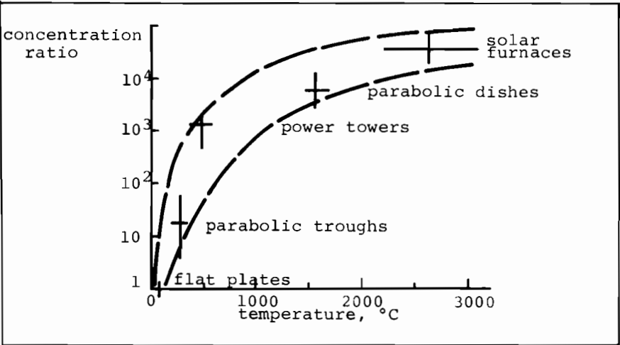
FIGURE 3A. Temperatures achieved by concentrator collectors
