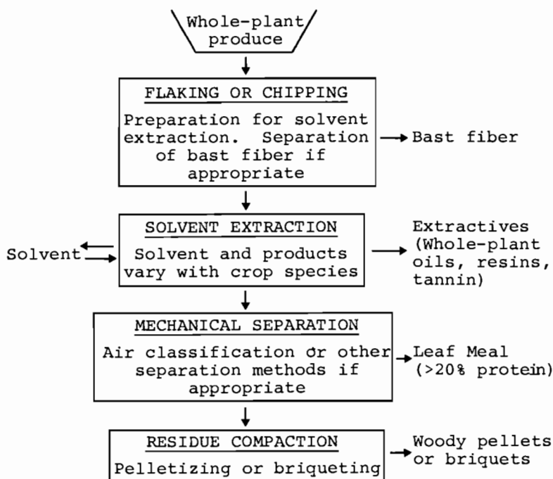
FIGURE 4. Multi-use botanochemical Primary Processing Subsystem
