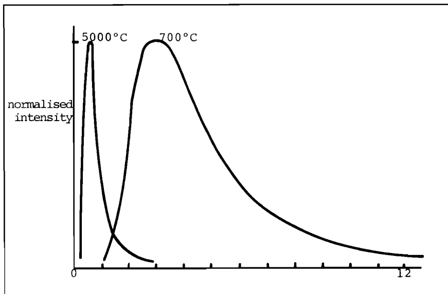
FIGURE 2A. Blackbody radiation from sources at the solar temperature and at the focus of a highly concentrating collector
