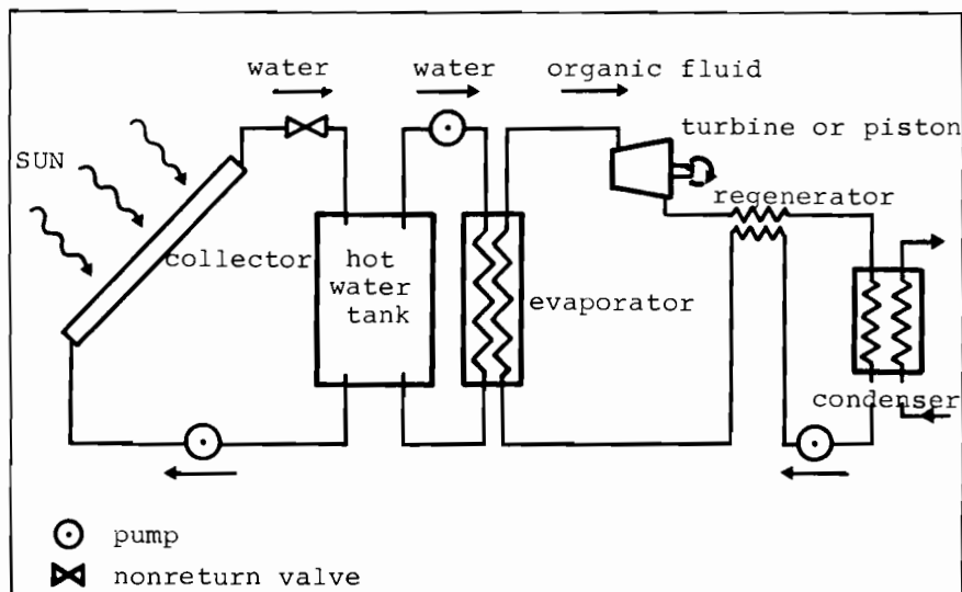
FIGURE 8. The fluid cycles for driving a heat-engine with solar energy. (Evaporator and hot water storage tank may be combined, and the organic fluid may even circulate through the collector to eliminate some heat exchangers).
