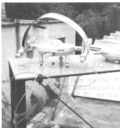
FIGURE 3. Diffusometer
