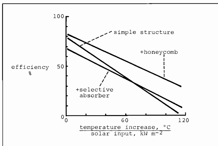
FIGURE 1B. Performance curves of some typical collectors with single glass covers, and the improvements shown
