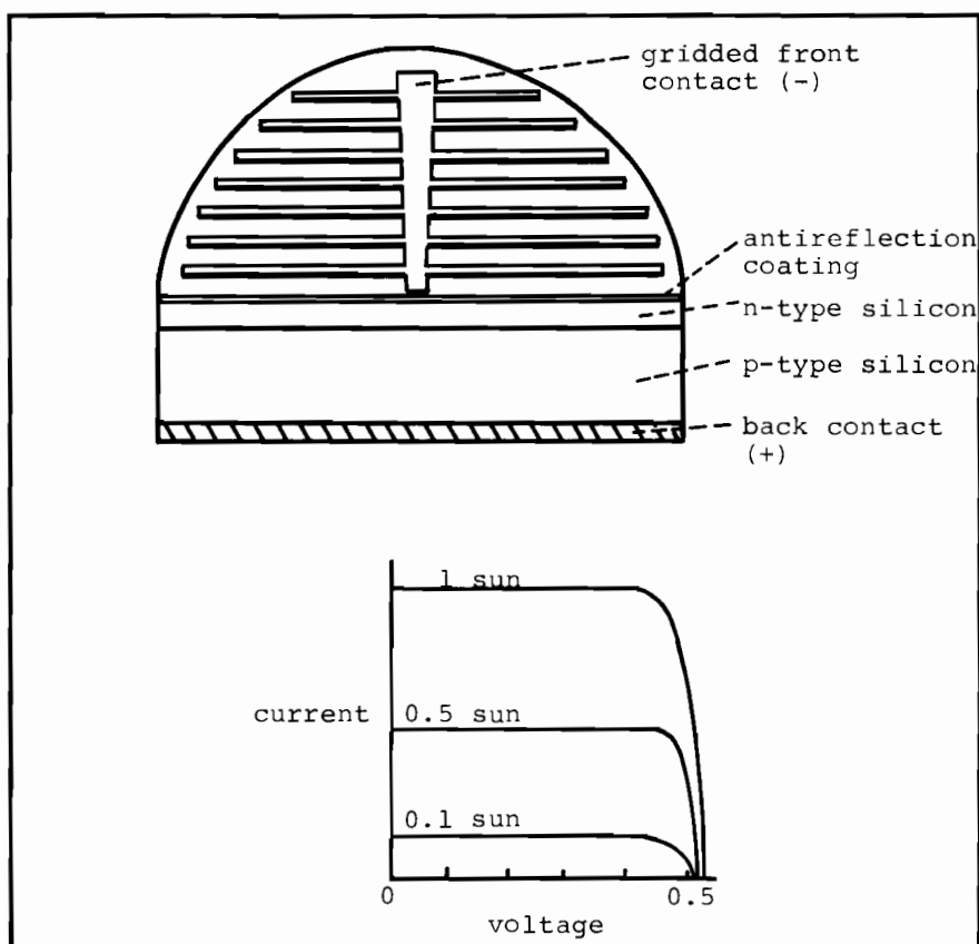
FIGURE 4A. Schematic cross-section of a p-n junction silicon solar cell. The silicon wafer is 0.3-0.5 mm thick, with a diameter of 75-100 mm.
