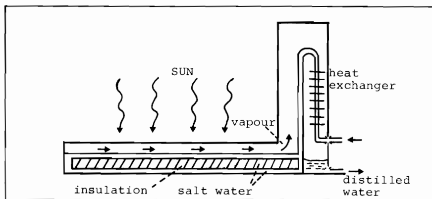
FIGURE 6B. Chimney still
