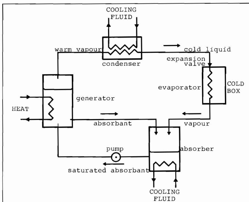
FIGURE 9. Continuous cycle refrigeration system using the absorption method. If heat is provided at 80^{\circ}\text{C} and cooling fluid at 30^{\circ}\text{C} , then 0^{\circ}\text{C} can be produced in the cold box with a coefficient of performance of 0.3
