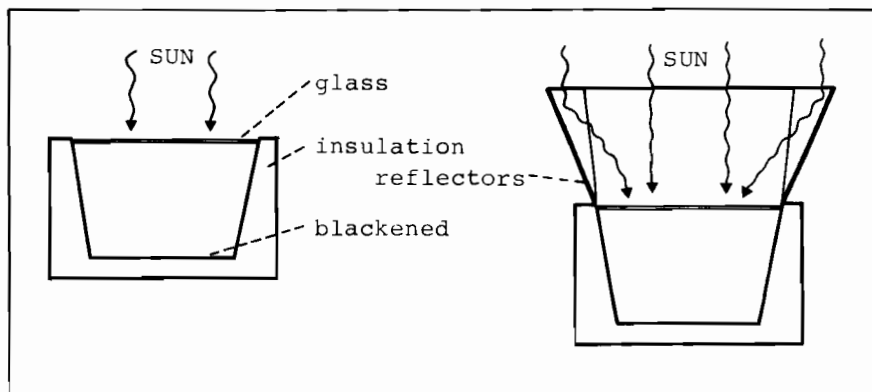
FIGURE 5. Simple solar ovens
