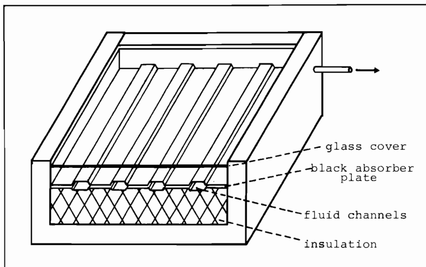
FIGURE 1A. Schematic cross-section through a simple flat-plate collector
