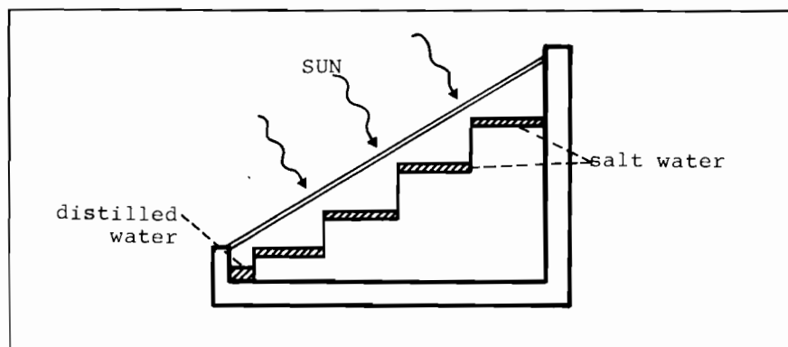
FIGURE 6A. Stepped basin still
