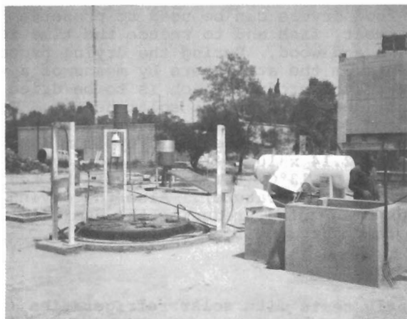
FIGURE 8. Digester of 15 \text{ m}^3
