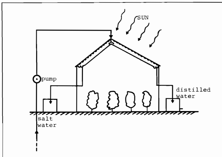
FIGURE 7. Solar still and greenhouse combined
