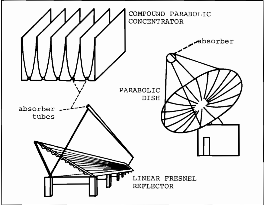
FIGURE 3B. Some practical concentrator collectors. The parabolic dish tracks on two axes, the Fresnel mirror strips track together, and the compound parabolic array is fixed
