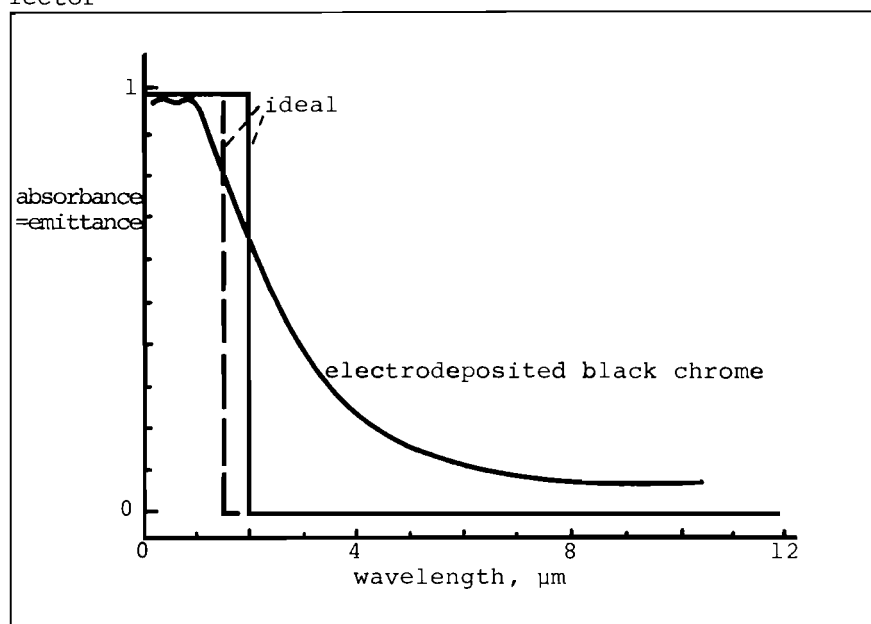
FIGURE 2B. Absorptance and emittance of ideal selective absorbers compared with that of a simple practical coating
