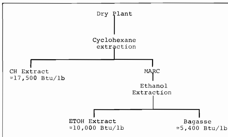
FIGURE 1. Hydrocarbon extraction scheme by the Arizona method
