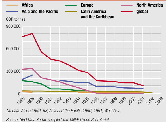
Figure 4: Consumption of chlorofluorocarbons (tonnes of ozone depleting potential) by region and global, 1988–2002
