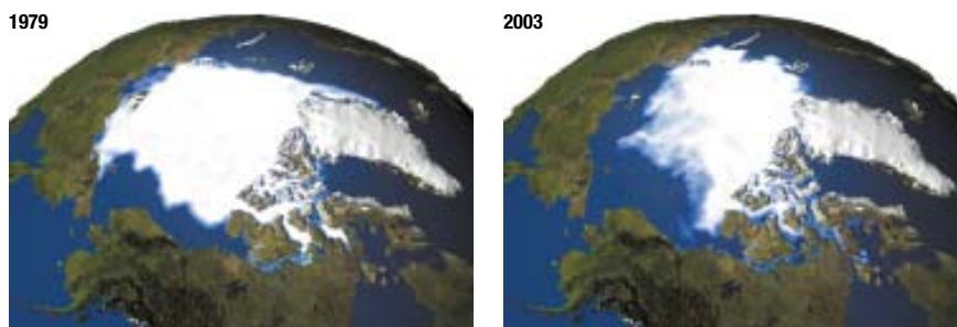
Figure 1: Dramatic changes in Arctic sea ice since 1979. The loss of Arctic sea ice may be caused by warming Arctic temperatures that result from greenhouse gas build-up in the atmosphere.
