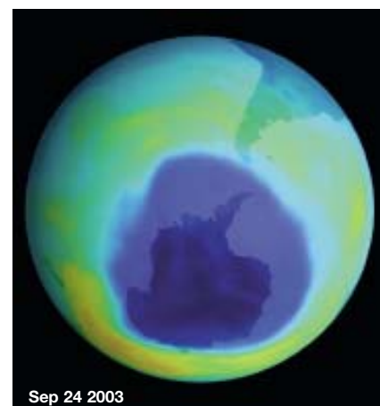
Figure 3: The 2003 ozone hole over Antarctica dark blue denoting high levels of ozone depletion was very large, close to the all-time record.
