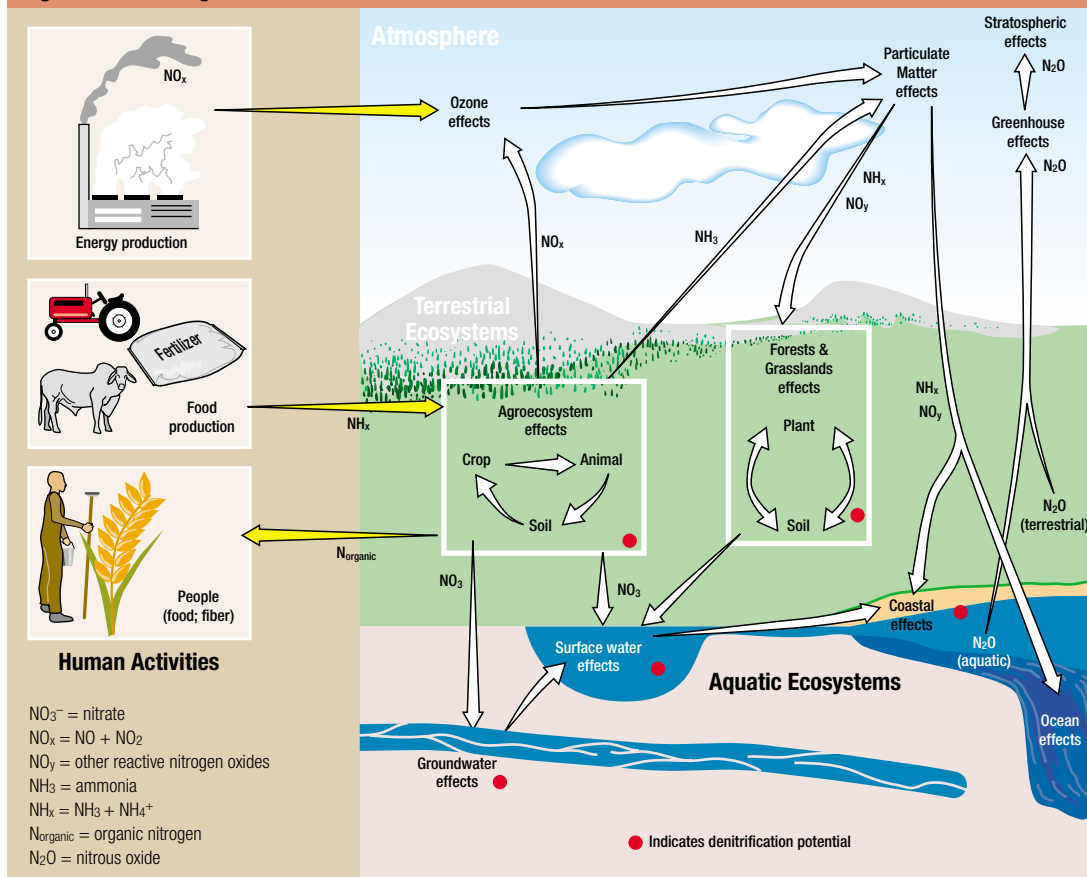
Figure 1: The nitrogen cascade
