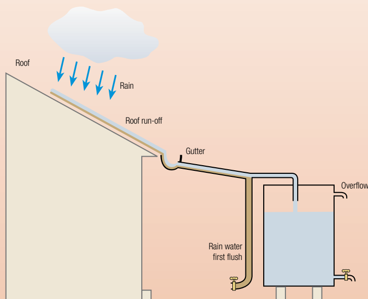
Diverter for the first flush from roof run-off
