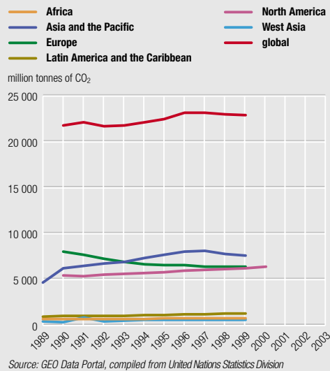
Figure 2: Total carbon dioxide emissions (million tonnes of CO 2 ) by region and global, 1989–2000
