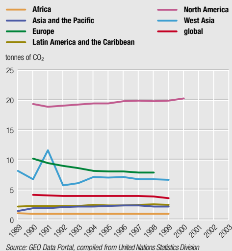
Figure 3: Total carbon dioxide emissions (tonnes of CO 2 ) per capita by region and global, 1989–2000
