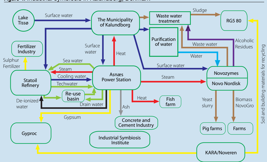
Figure 4: Industrial symbiosis in Kalundborg, Denmark
